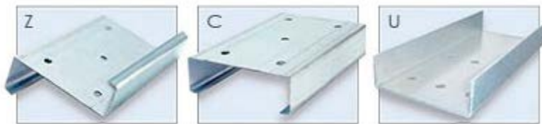
Figure 8. C, Z, and U purlins for solar racking
