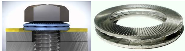
Figure 1. Wedge-lock washers
